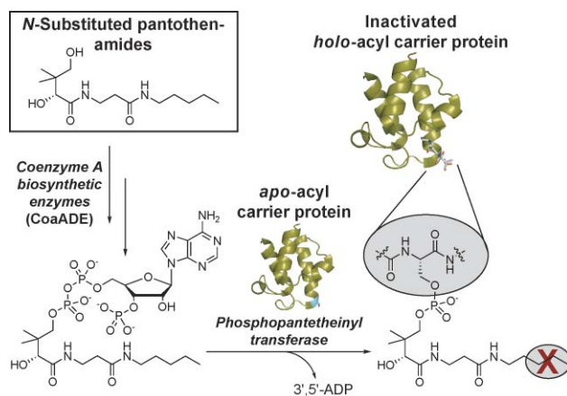
Scheme 1 N -Substituted pantothenamides (such as N -pentyl pantothenamide shown above) act as antimetabolites by forming coenzyme A analogues which do not contain the essential terminal thiol group of natural CoA. These analogues subsequently transfer inactive prosthetic groups to the acyl carrier proteins that are involved in fatty acid metabolism, thereby blocking these processes.
